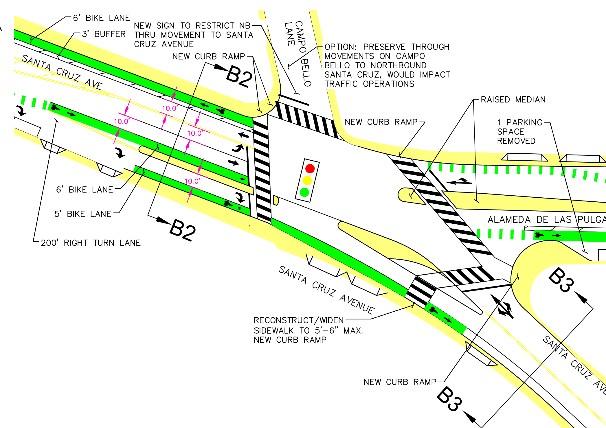
ALTERNATIVE B ONE TRAVEL LANE IN EACH DIRECTION BIKE LANE SOUTH OF Y
