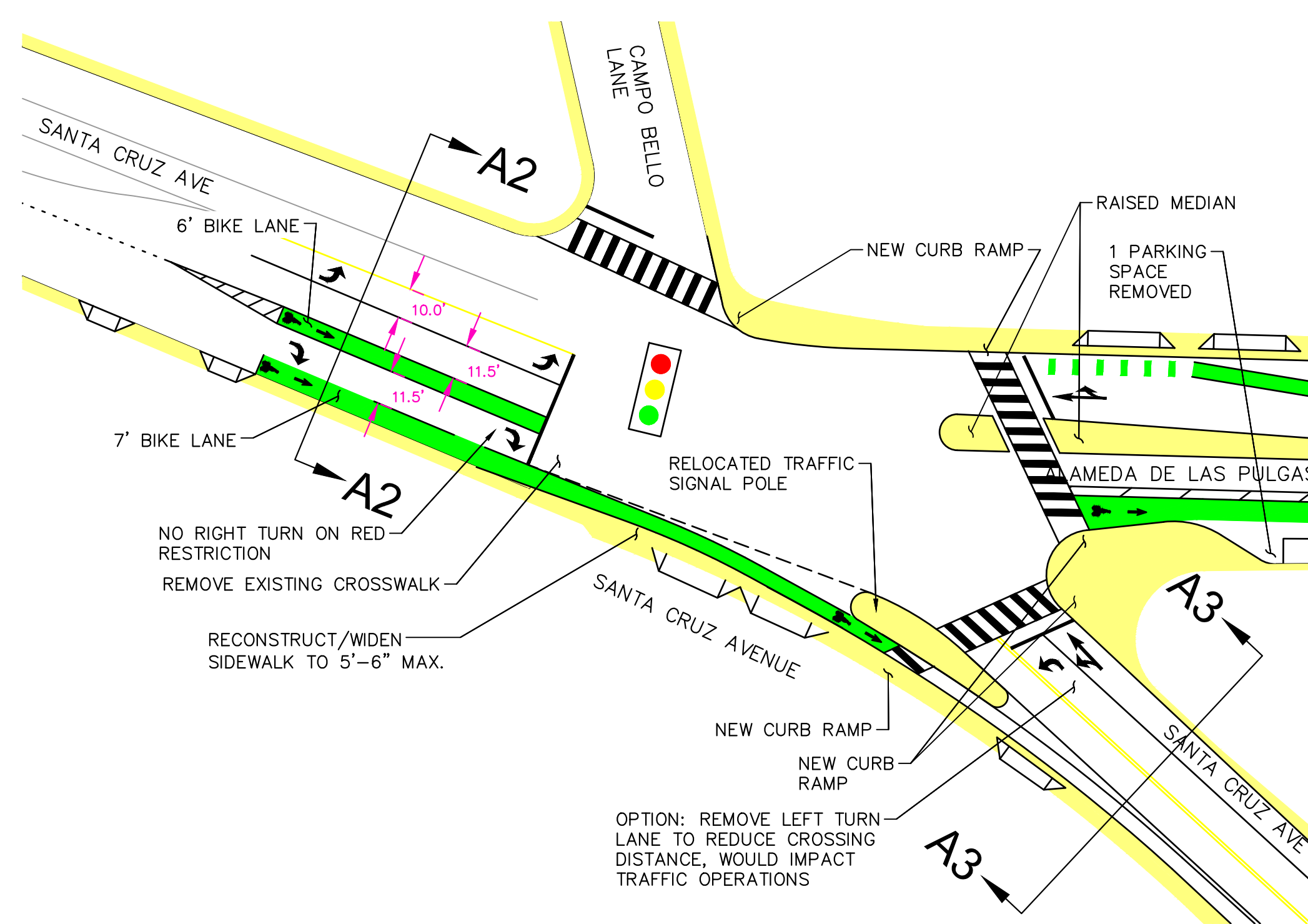
ALTERNATIVE A TWO TRAVEL LANES IN EACH DIRECTION NO BIKE LANE SOUTH OF Y
