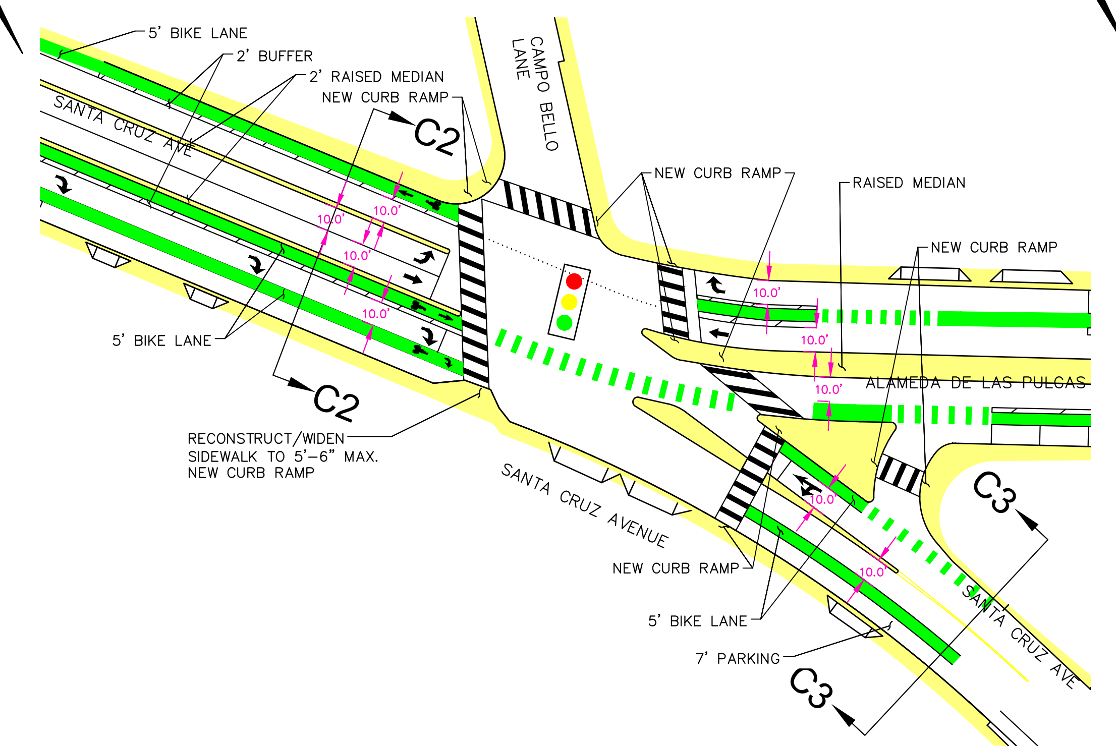
ALTERNATIVE C TWO TRAVEL LANES NB AND ONE TRAVEL LANE SB BIKE LANE SOUTH OF Y
