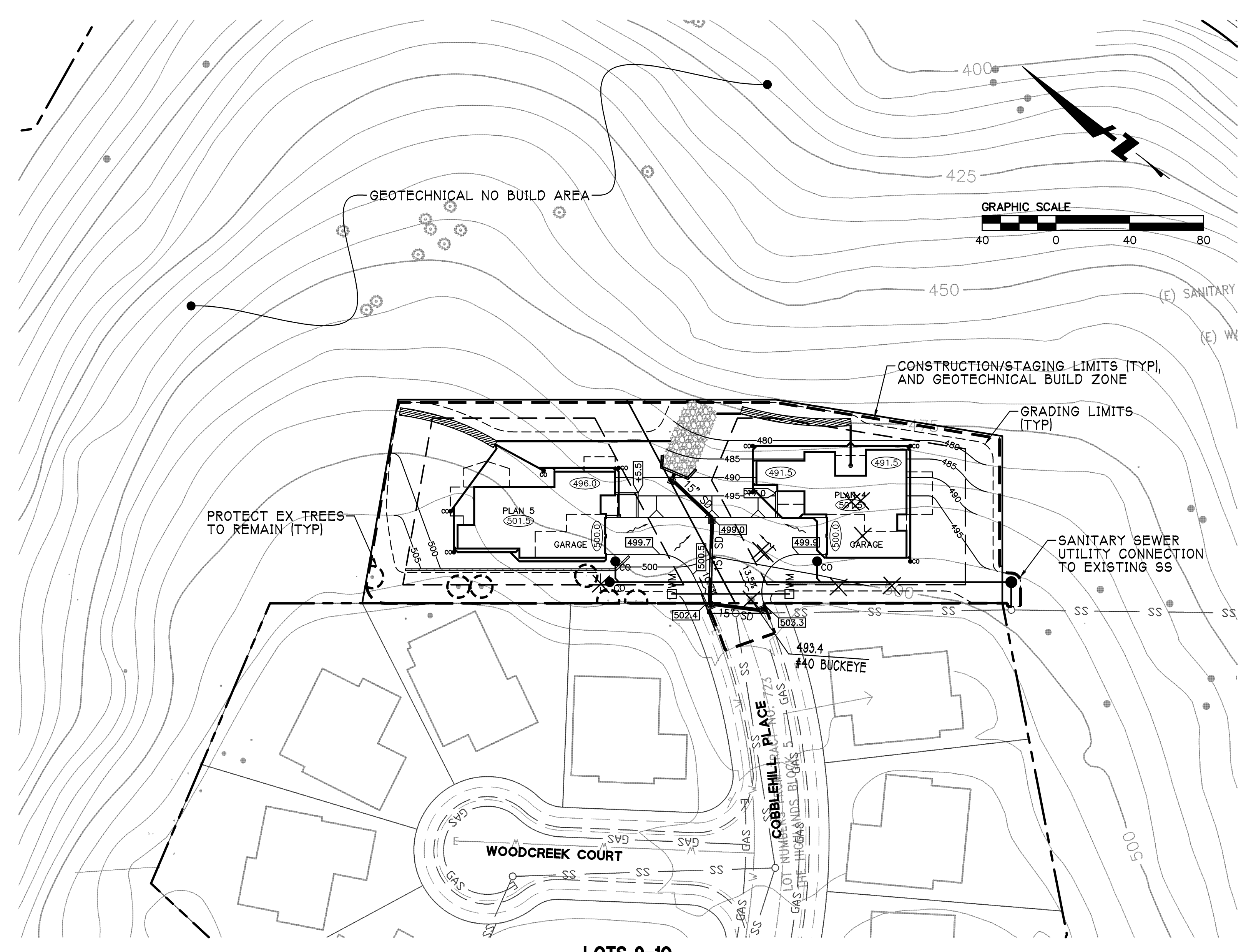
LOTS 9-10 CLEARING, CONSTRUCTION, AND GRADING LIMITS PLAN SCALE: 1"=40'
