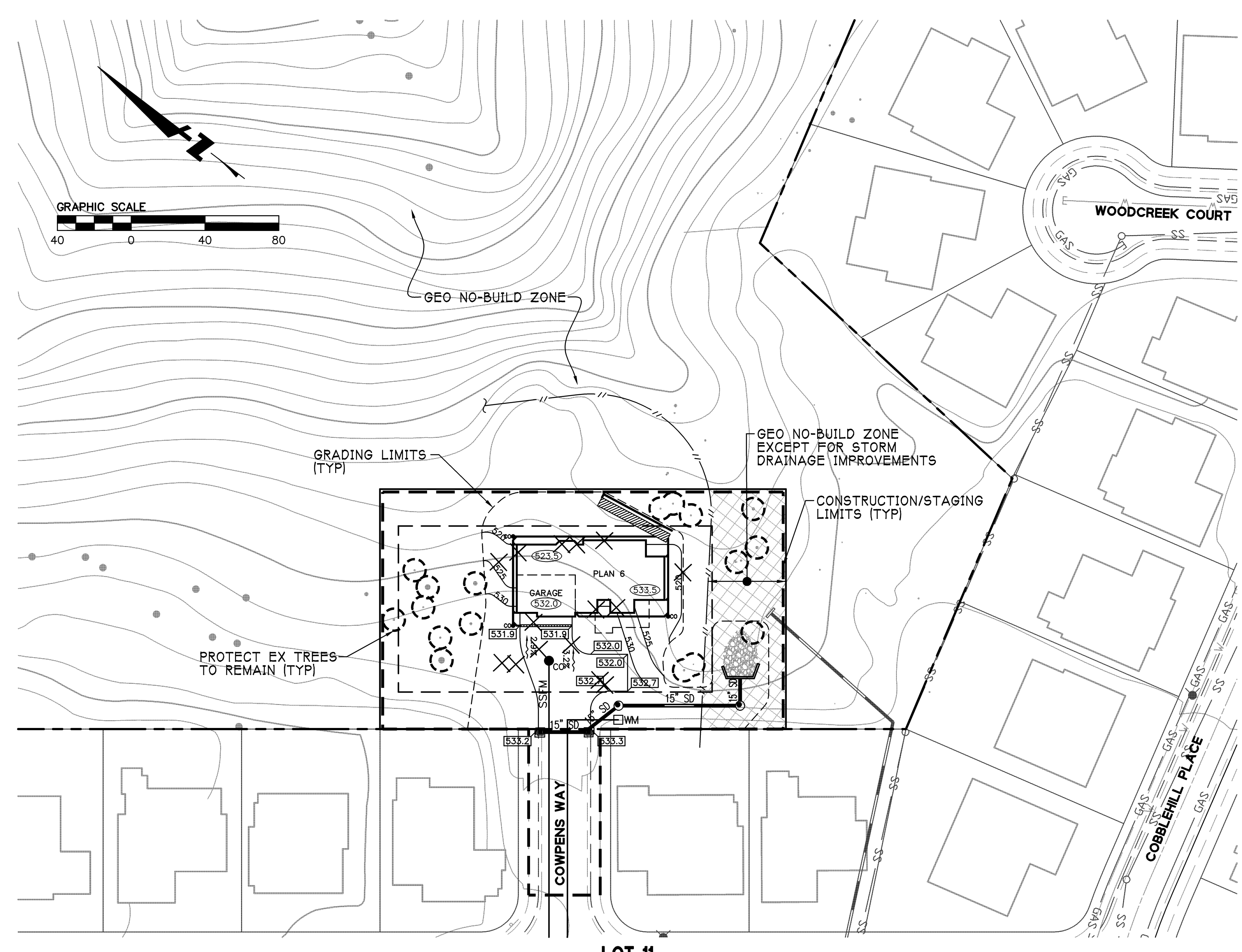
LOT 11 CLEARING, CONSTRUCTION, AND GRADING LIMITS PLAN SCALE: 1"=40'
